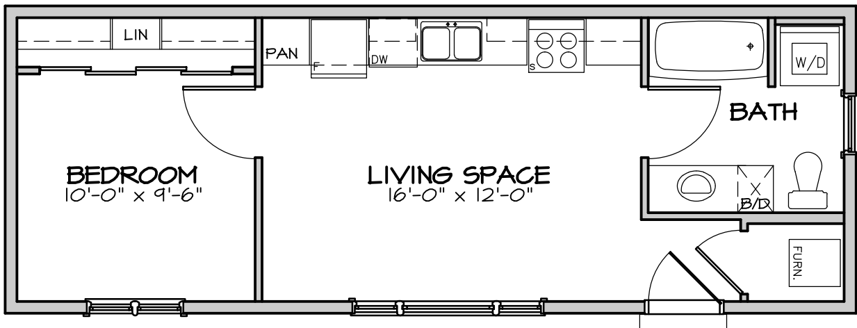
GROUND FLOOR PLAN 468 SQ. FT.
